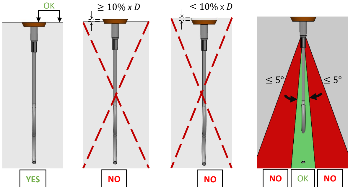
Figure 4 Correct placement of nailing plate.
