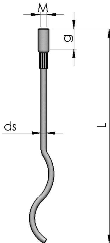
Figure 9 Transport anchor with rebar long wave sketch.
