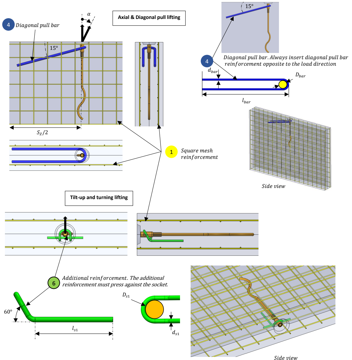
Figure 7 Reinforcement in the concrete wall.
