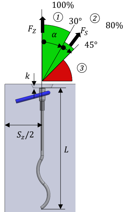
Axial & Diagonal pull lifting
