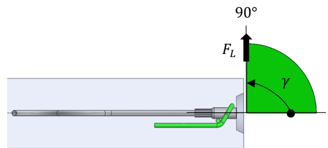
Tilt-up and turning lifting
