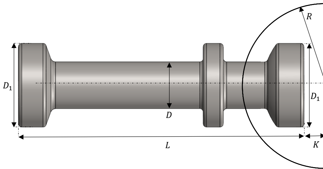
Figure 12 Automation spherical anchor sketch.
