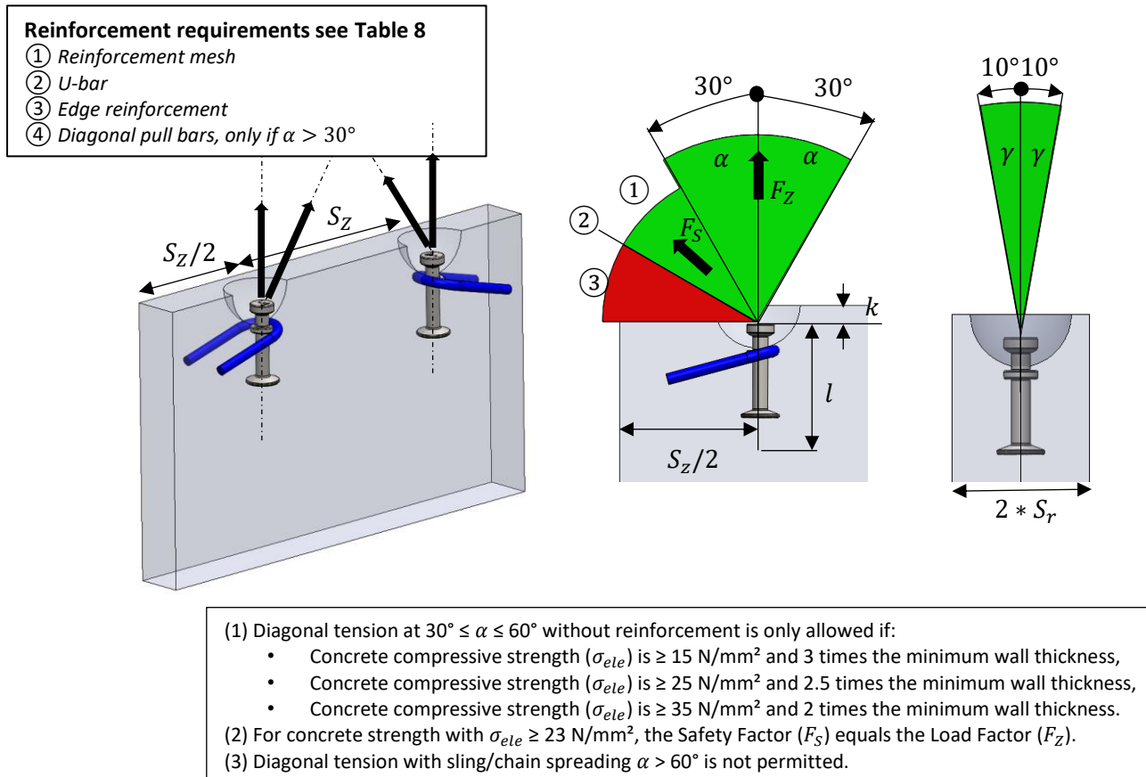
Figure 10 Reinforcement requirements.
