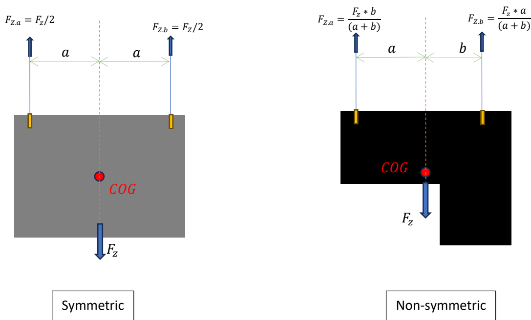
Figure 8 Calculation symmetric and non-symmetric loading element.
