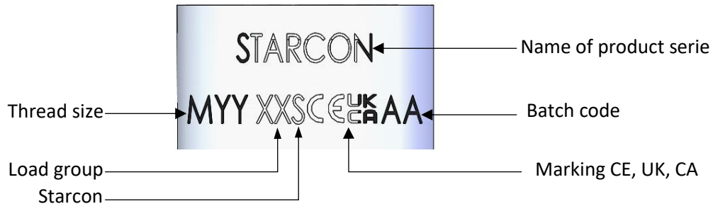
Figure 2 Marking on the cylinder of the transport anchor.
