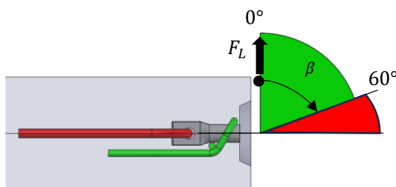
Tilt-up and turning lifting
