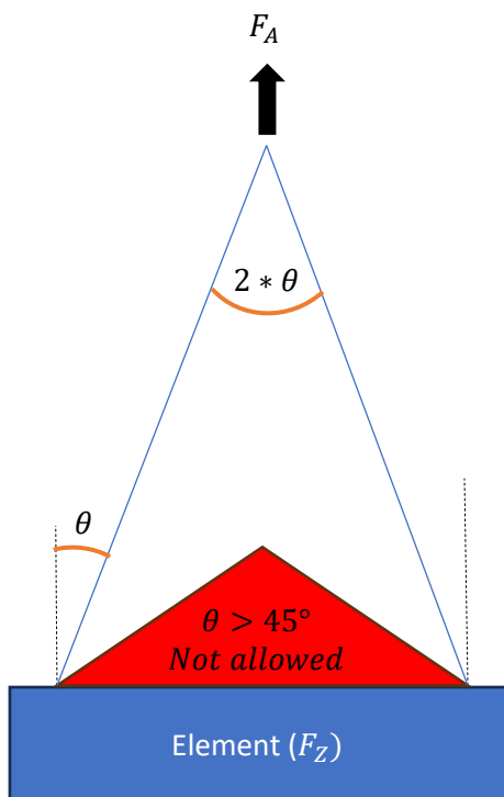
Figure 5 Sling angle factor illustration.
