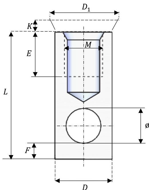
Figure 10 Lifting socket solid material sketch.
