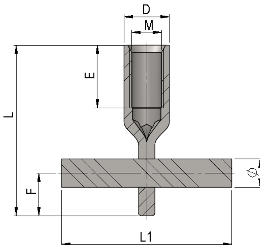
Figure 9 Transport anchor with cross pin sketch.
