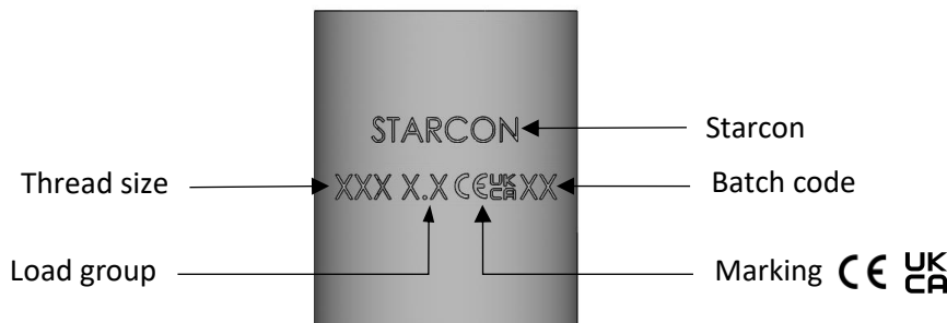
Figure 2 Marking on the cylinder of the transport anchor with cross pin.
