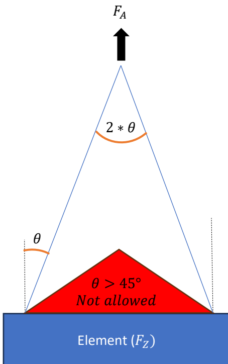
Figure 5 Sling angle factor illustration.
